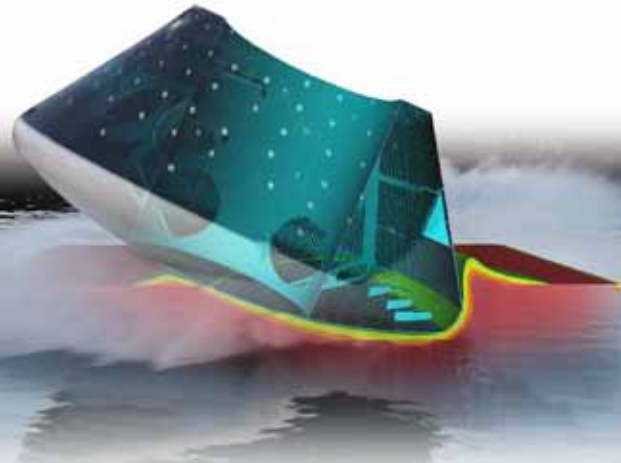
Crew module water landing simulation.
